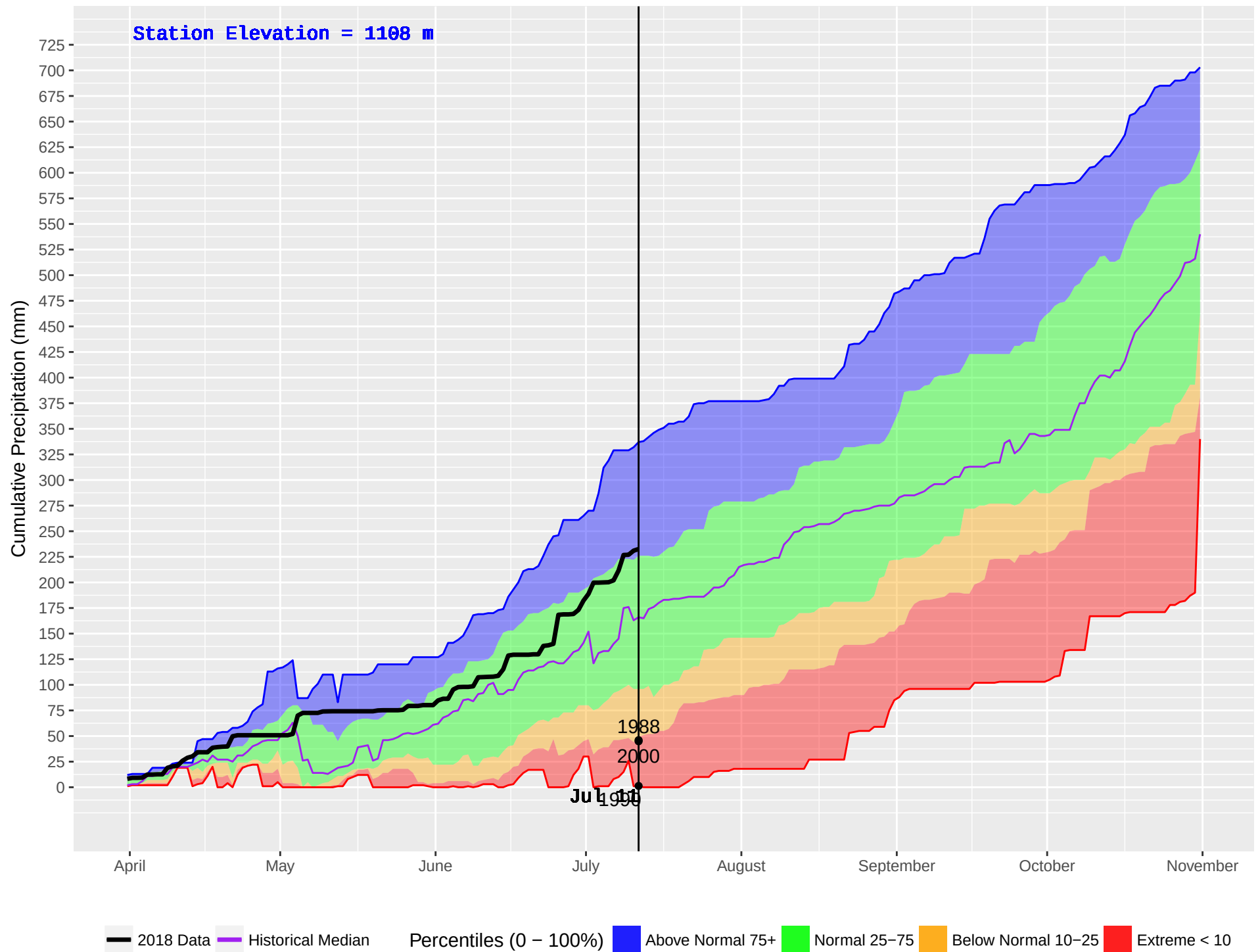
MATHEW (263) : Historical (1987–2016) and Current (2018) Noon Cumulative Precipitation
